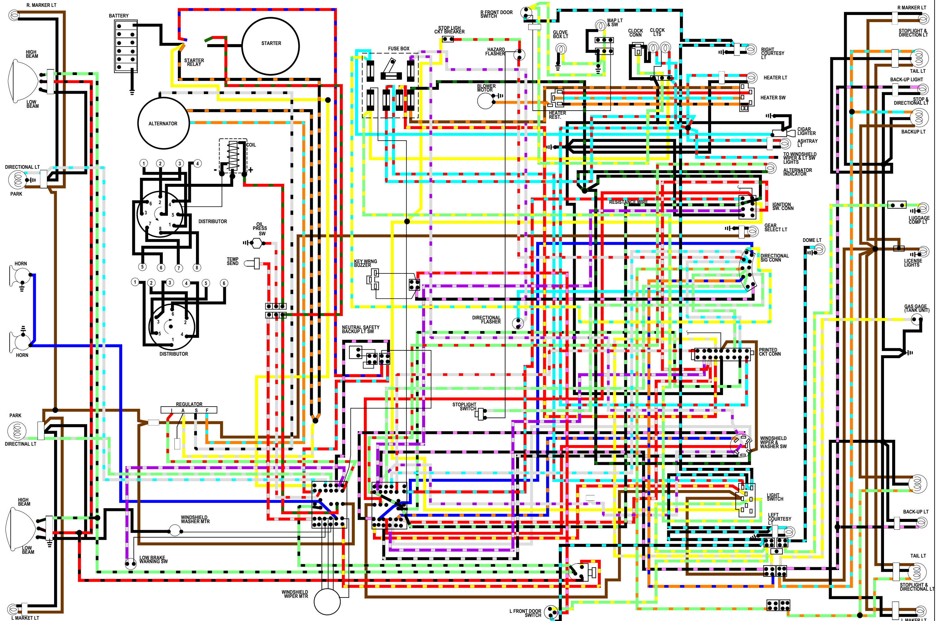
1972 MUSTANG CIRCUIT DIAGRAM
